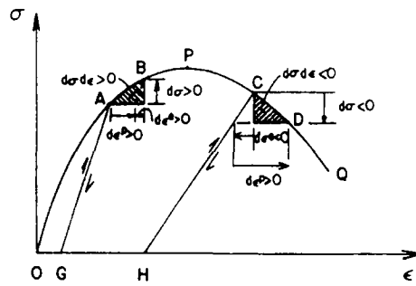
Fig. 2. Features of softening behavior.
