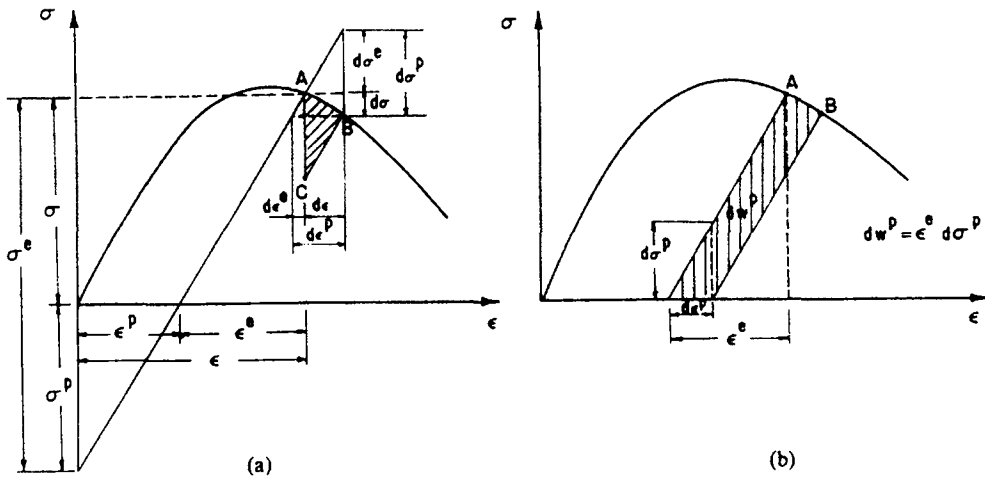
Fig. 5. Schematic description of plasticity formulation based on Il'yushin's postulate: (a) stress and strain increments; (b) plastic work increment.
